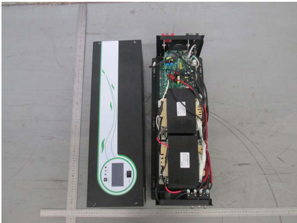
Fig. 5 –Inside view
